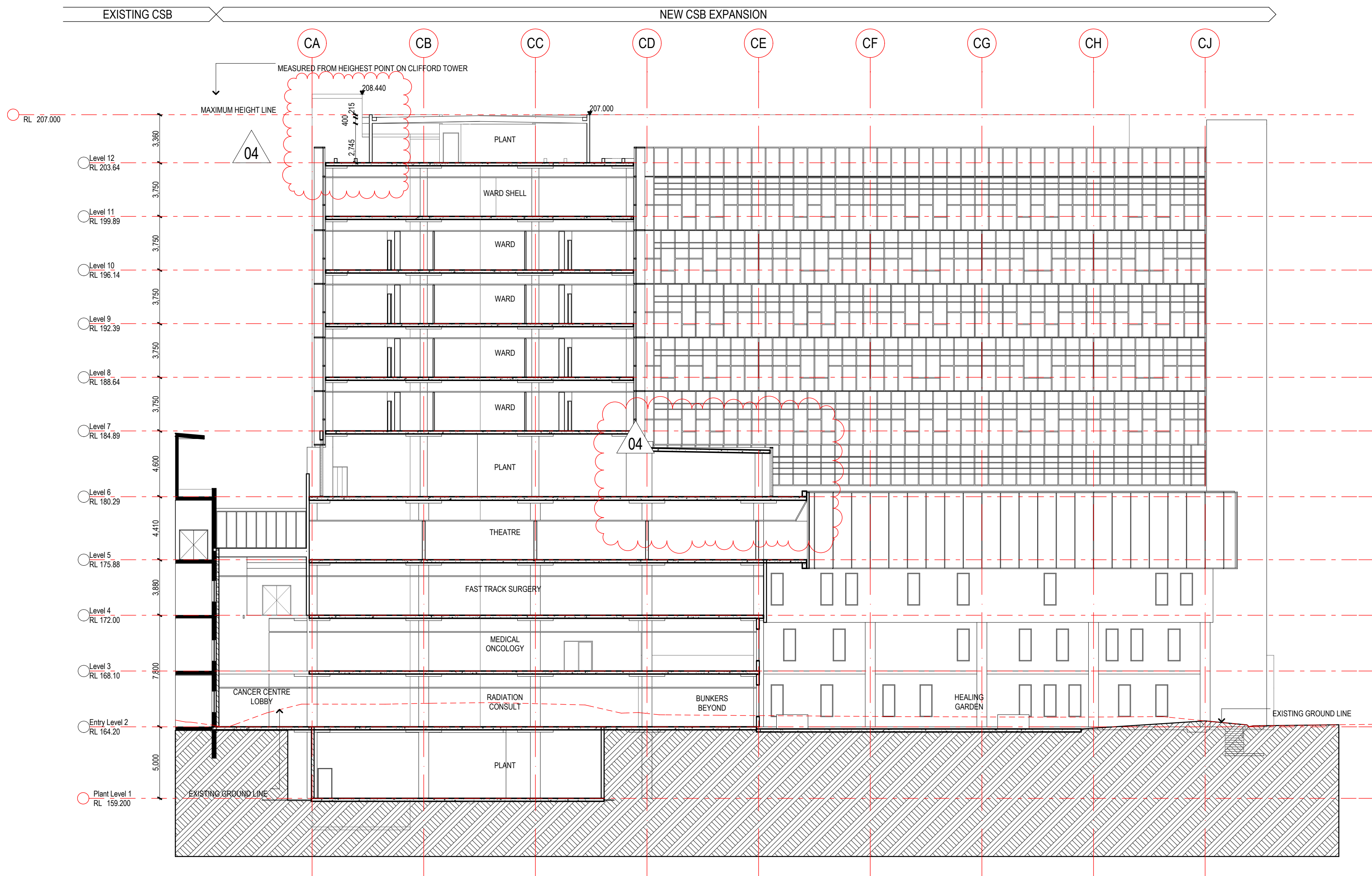
C-F SECTION F SCALE 1:200
