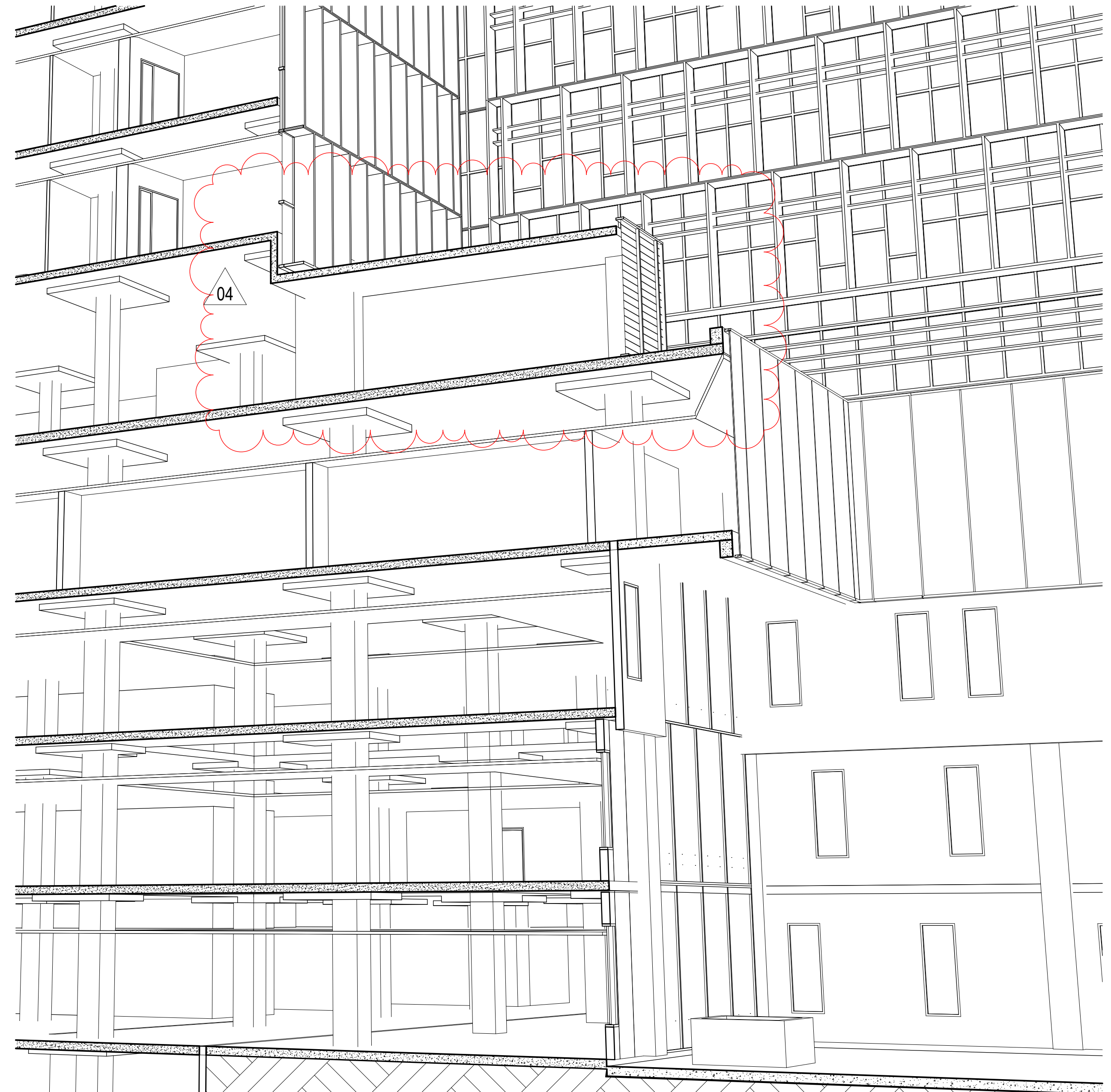
3 3D SECTION C-F SCALE 1:11.96
